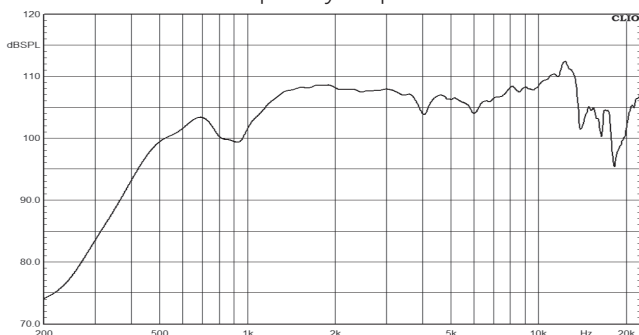
Frequency response
